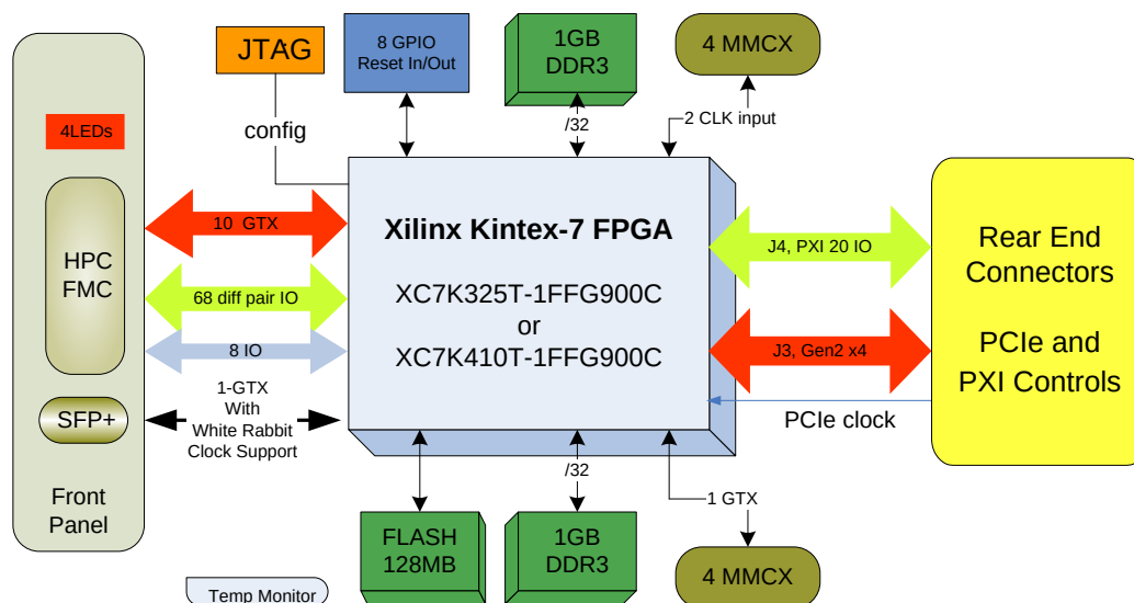
Figure 1: PXIe-700 Block Diagram
