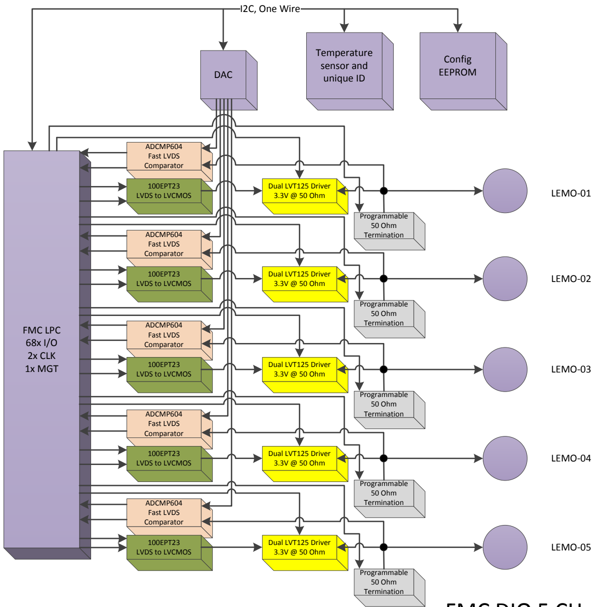
FMC DIO 5 CH FMC Digital I/O - 5 channels TTLA
