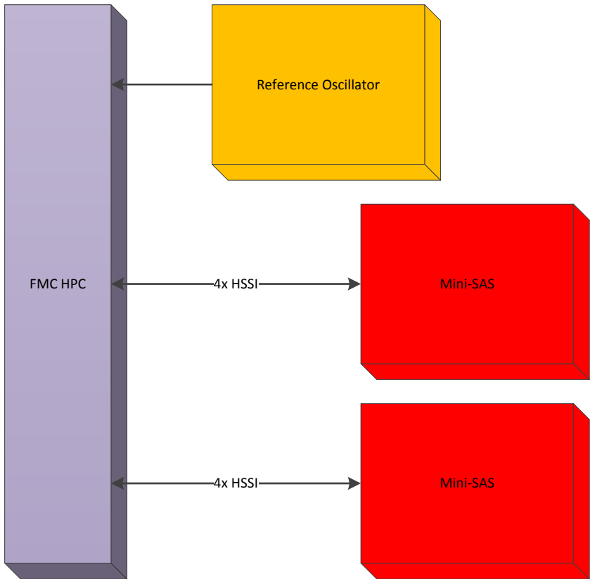
FM550 Two Channel mini-SAS I/O FMC
