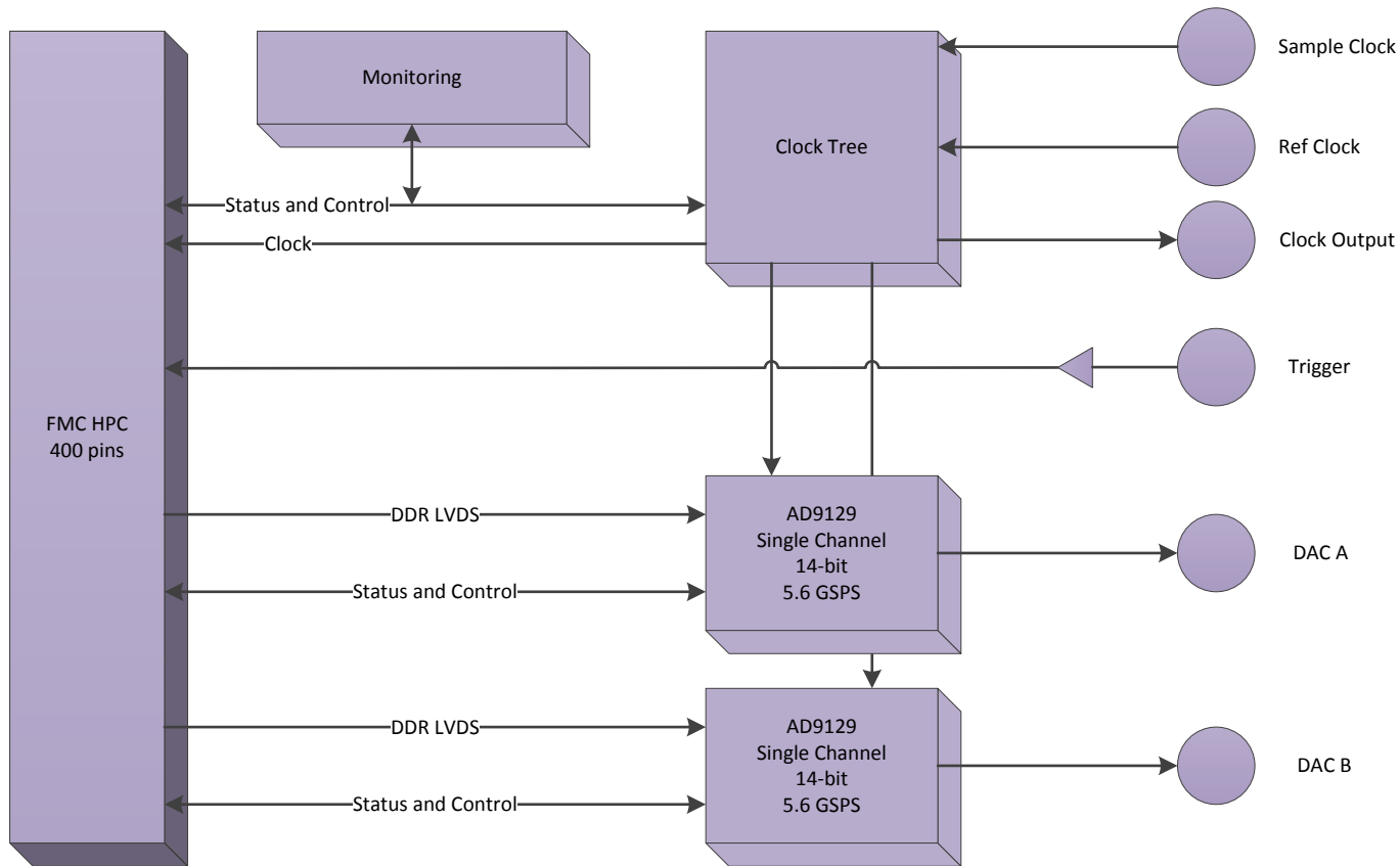
FMC230 Dual 14-bit 5.6Gsp/s D/A FMC VITA 57.1 Compliant
